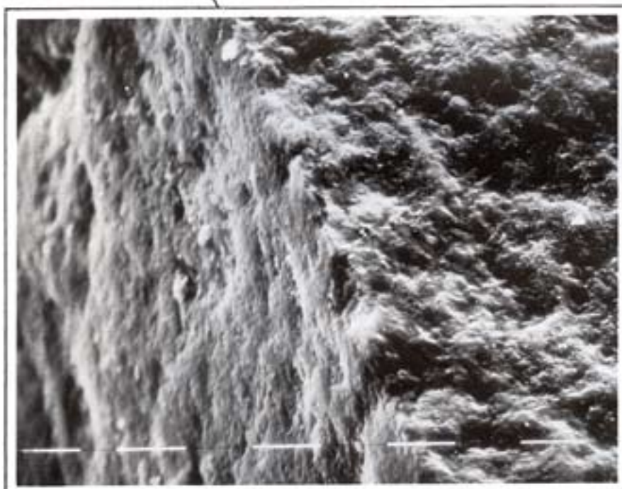
Ecaillage op vuursteen.Coating: Au. 1500 x vergroting. ————— = 10 \mu .
